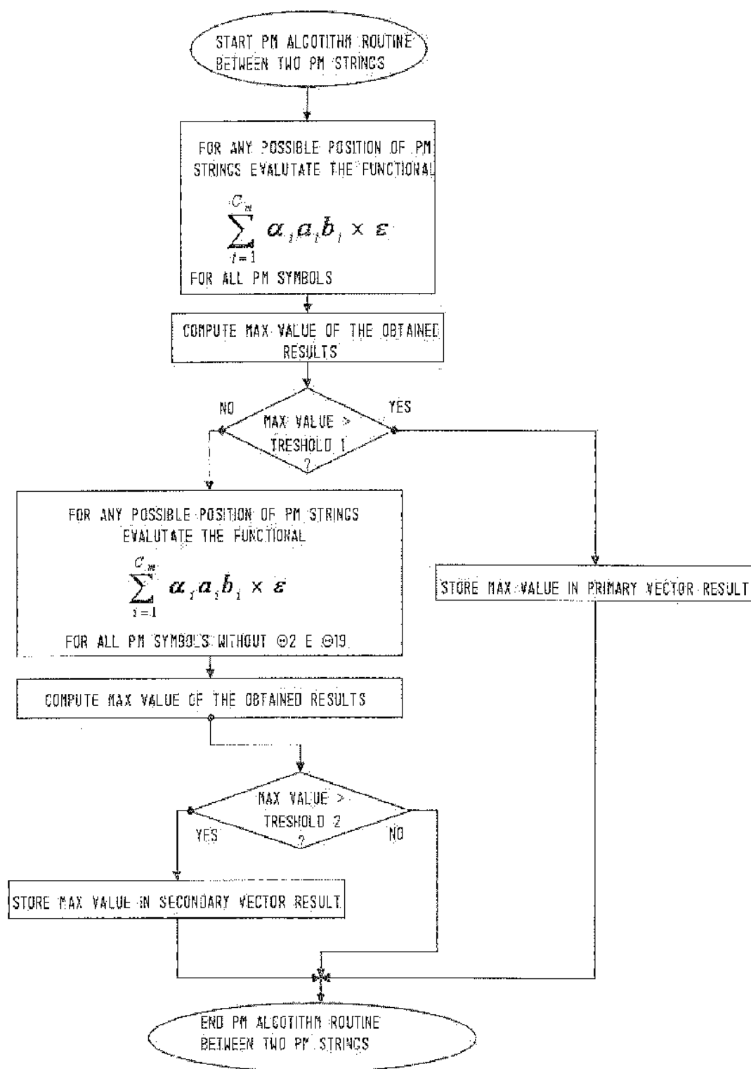
Fig 8.b Block Diagram describing Plate Matching algorithm routine between two PM strings
